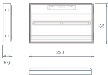
TOLEDO IP 42
